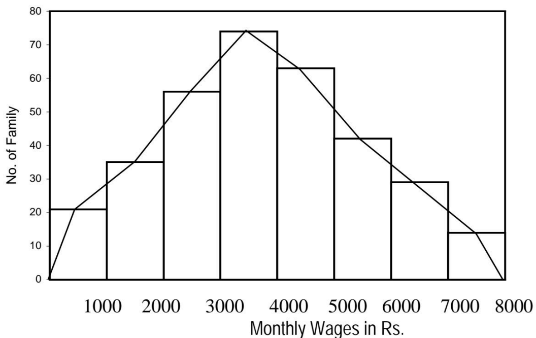
FREQUENCY CURVE
