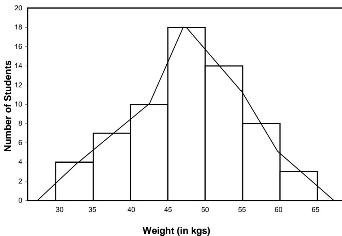
FREQUENCY POLYGON
