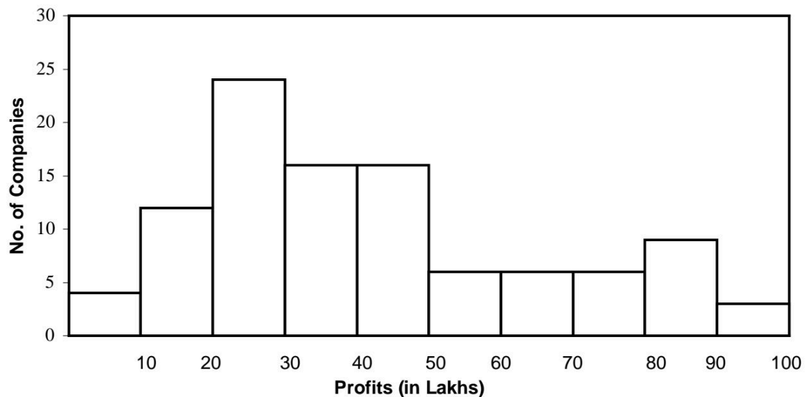
HISTOGRAM
